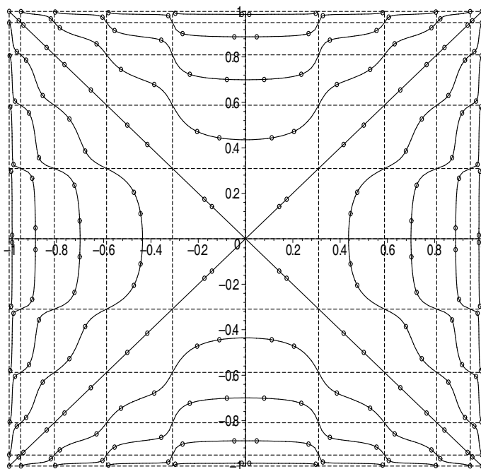
FIGURE 3. The projection to the (x, y) plane of curves of fixed points of type (F2) and (F3).
